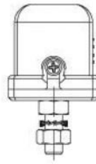
Indicative dimensions lamp - mm unit
